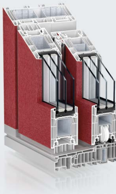
PremiDoor 76
